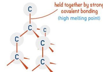
Carbon (diamond), C_{(s)}
